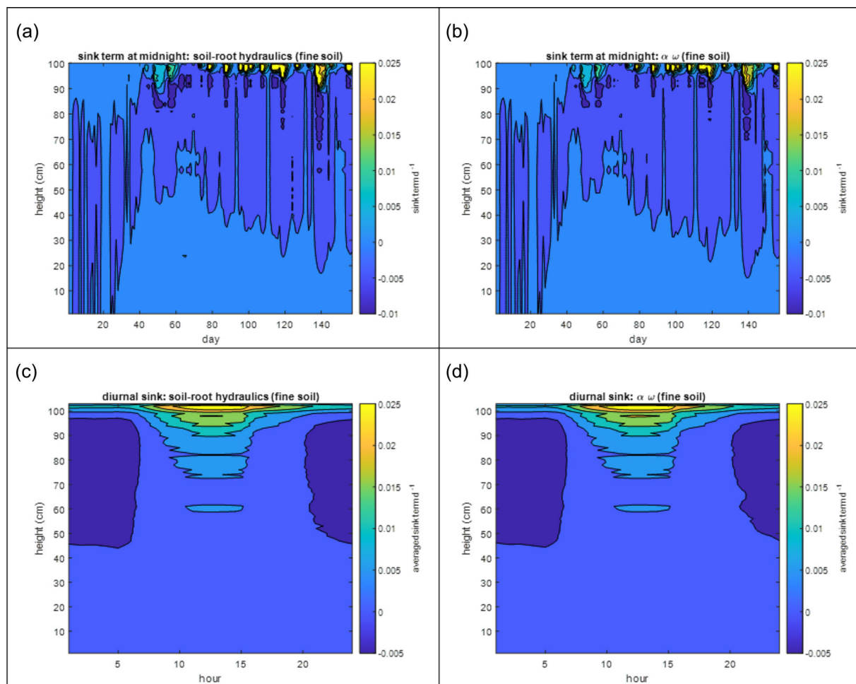
FIGURE 4 Simulated sink term distributions at midnight when the T_p = 0 in the fine-textured soil using the mechanistic soil–root hydraulic model (a), the mechanistically derived \alpha\omega macroscopic uptake functions (b), the average diurnal course of the sink terms simulated by the mechanistic soil root hydraulic model (c), and the mechanistically derived \alpha\omega macroscopic uptake functions (d).
