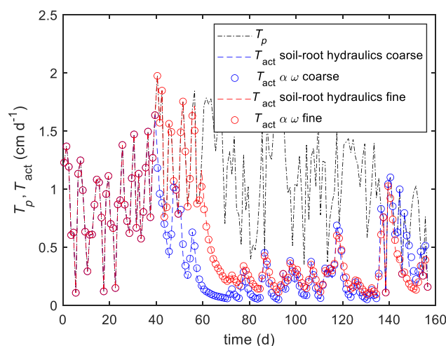
FIGURE 3 Potential ( T_p ) and simulated actual transpiration rates ( T_{act} ) at midday in the coarse- (blue) and fine-texture (red) soil using the soil root hydraulic model (dashed lines) and the model with mechanistically derived \alpha - \omega macroscopic uptake functions (open circles).
